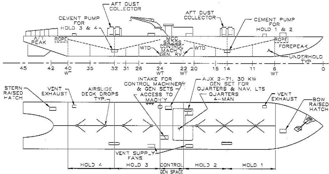
Cement Transporter 5300
