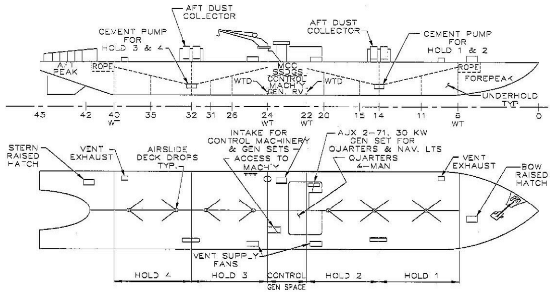
Cement Transporter 5300
